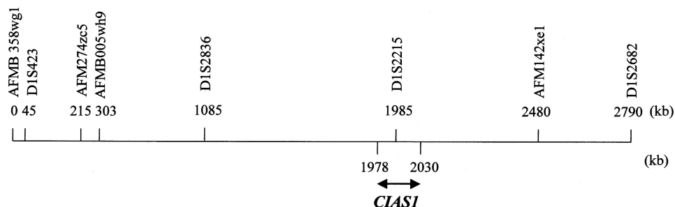
Figure 3 Physical map of the region surrounding the CIAS1 gene, between microsatellite markers AFMB358wg1 and D1S2682 (UCSC Human Genome Project Working Draft).
